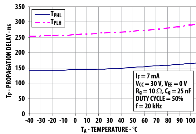
Figure 19 Propagation Delay vs. Temperature
