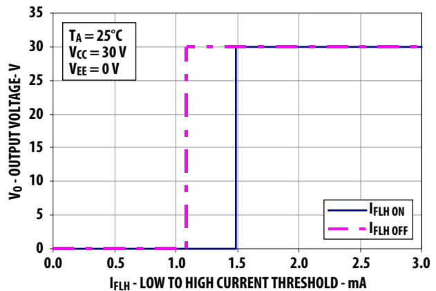
Figure 12 I_{FLH} Hysteresis
